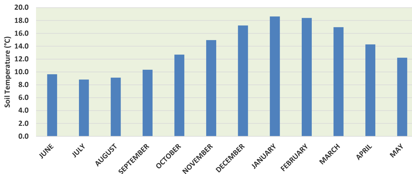
DTT Gibson - Average Monthly Soil Temperature
